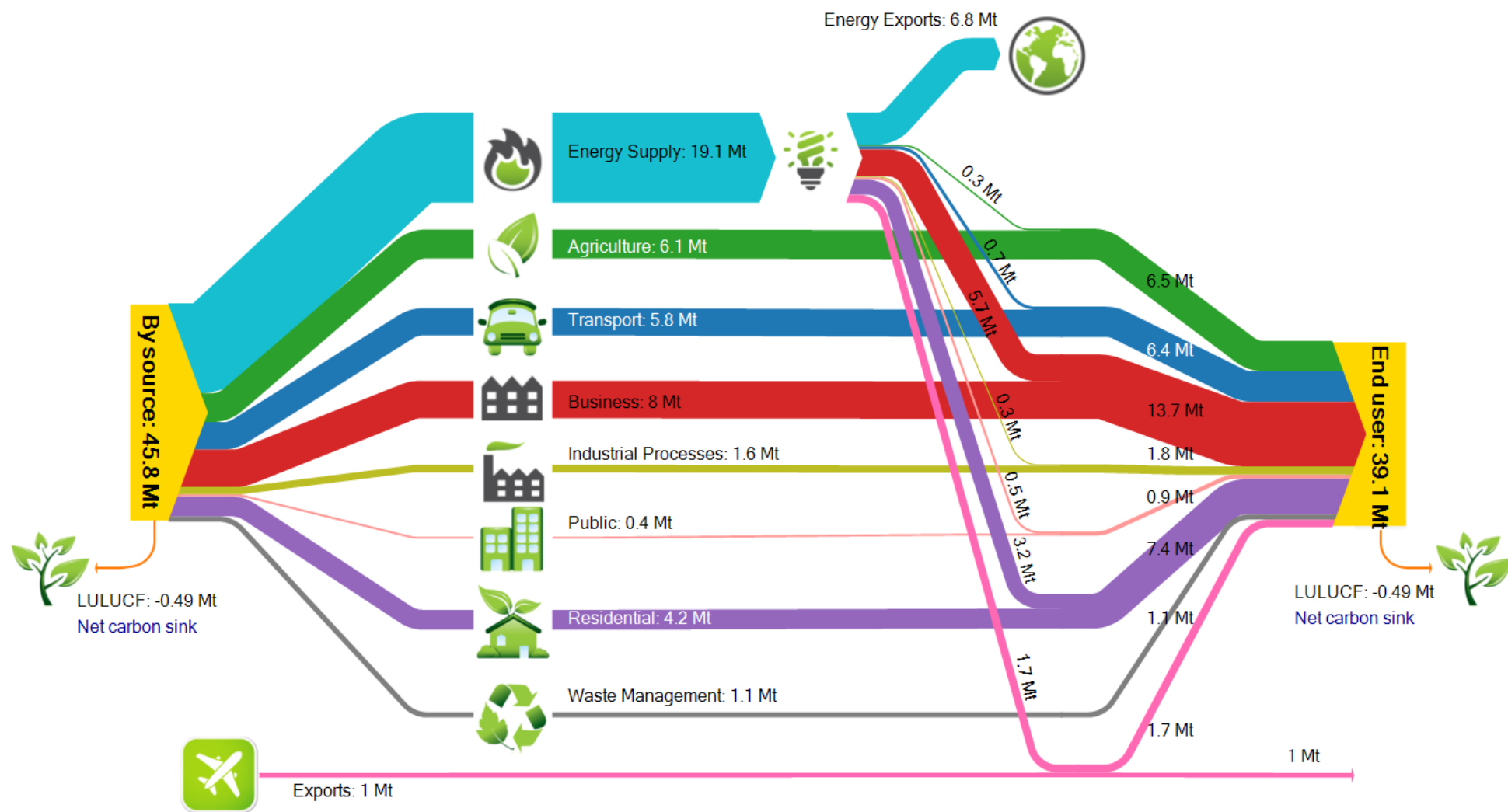
Figure 4.9 Sankey diagram showing By Source and End User 24 GHG emission transfers for Wales in 2012 (Mt CO 2 e) 25
